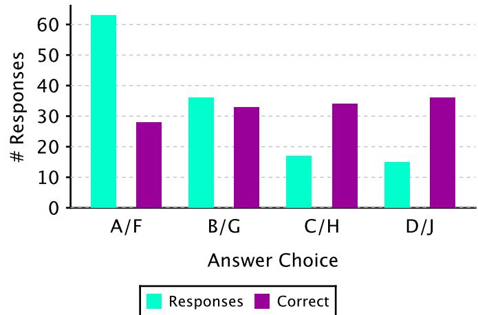
Answer Distribution
